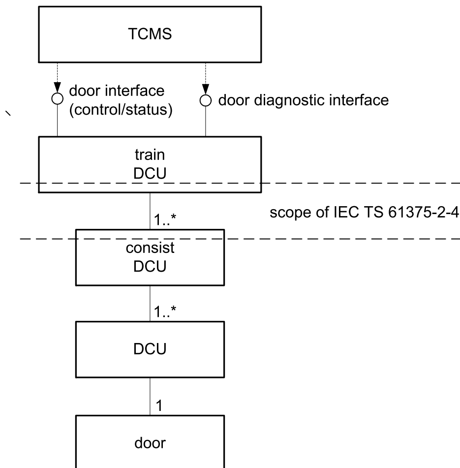
Figure 23 – Architecture of the door system
