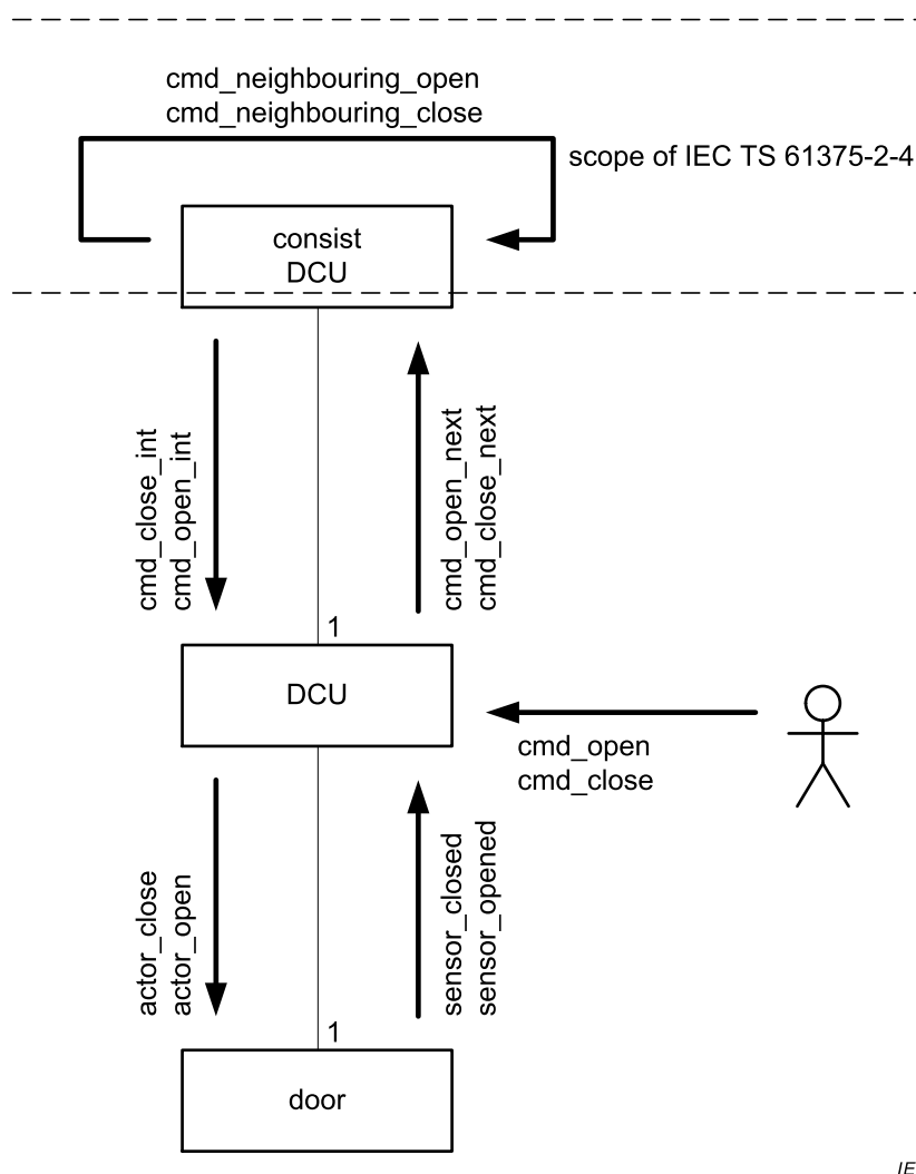
Figure 30 – Communication flow of triggers for neighbouring interconnecting doors
